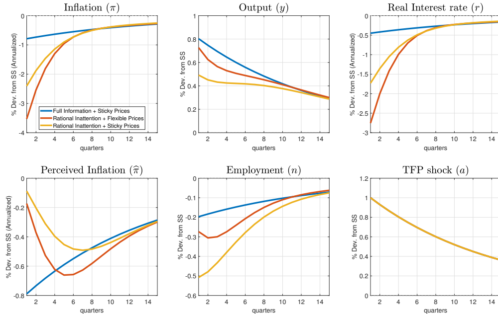
Figure 5: Dynamic Responses to a Technology Shock
